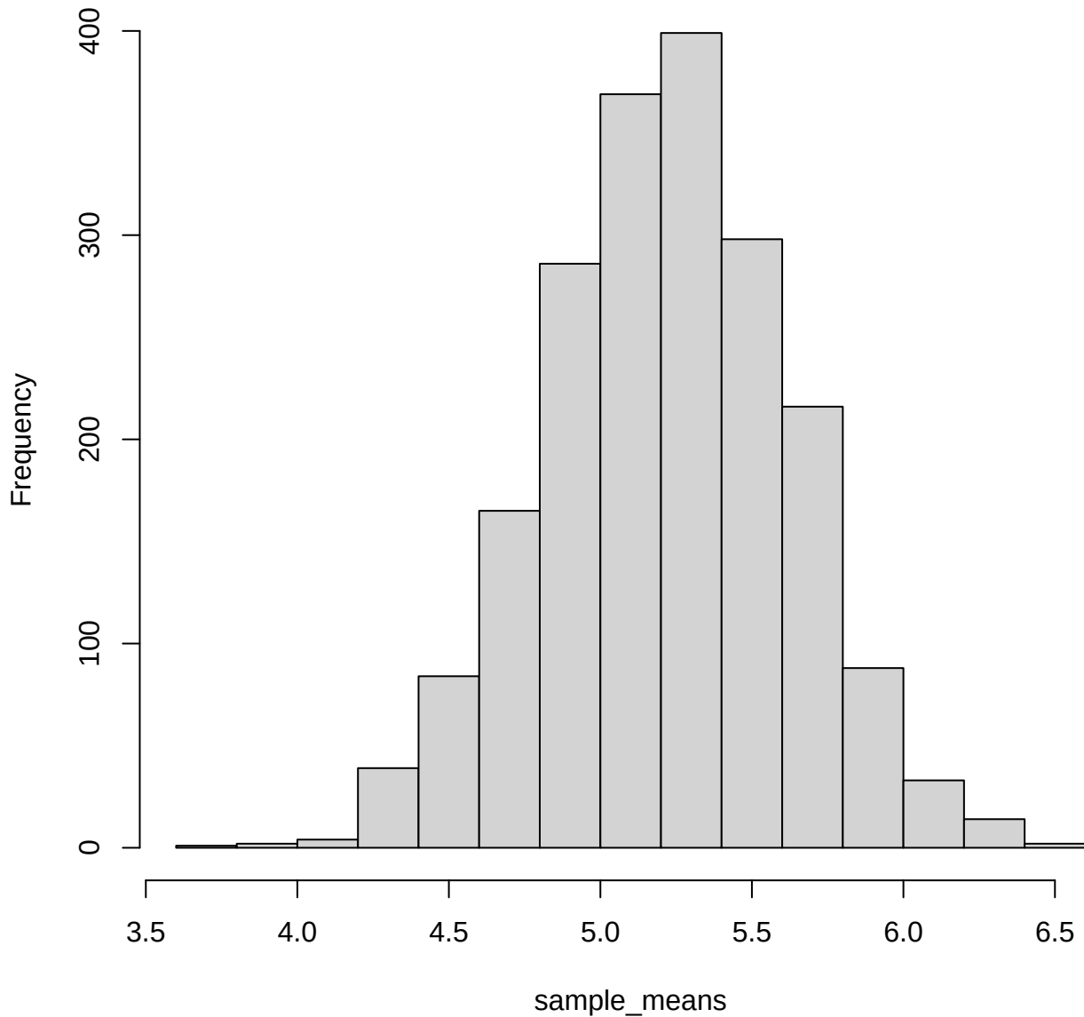
Histogram of sample_means
