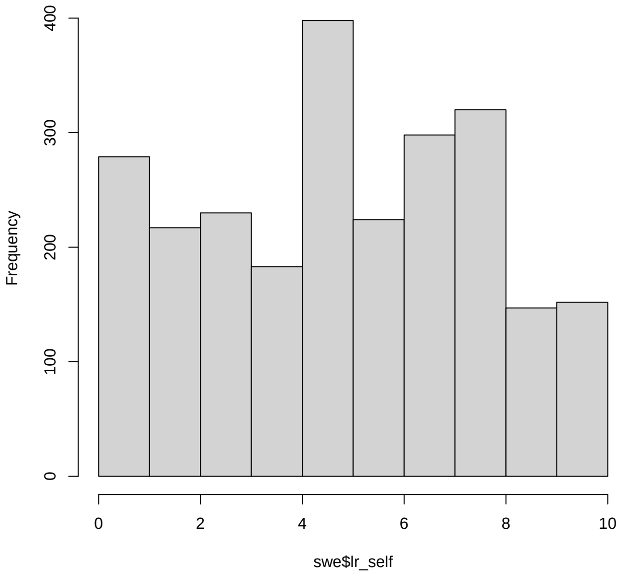
Histogram of swe$lr_self
